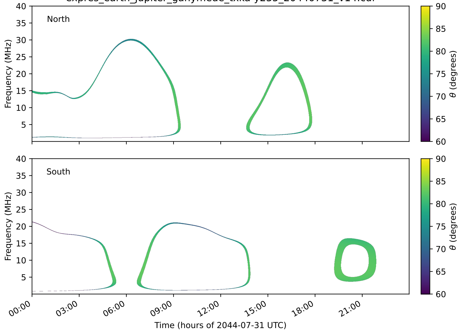
expres_earth_jupiter_ganymede_txka-y235_20440731_v14.cdf
