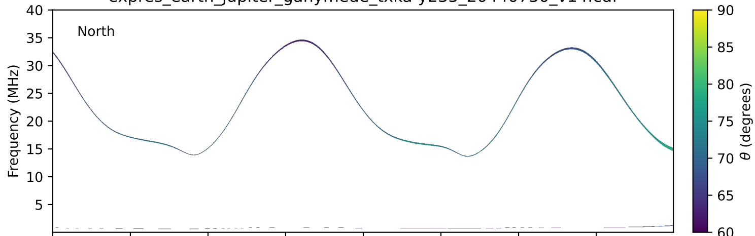
expres_earth_jupiter_ganymede_txka-y235_20440730_v14.cdf
