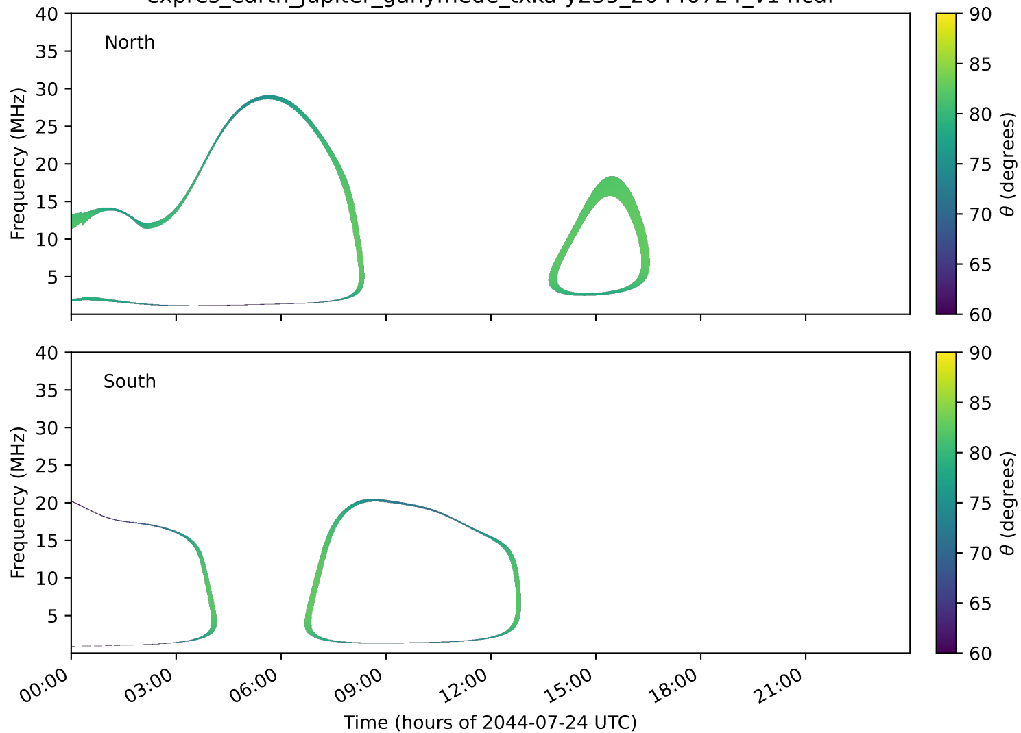
expres_earth_jupiter_ganymede_txka-y235_20440724_v14.cdf
