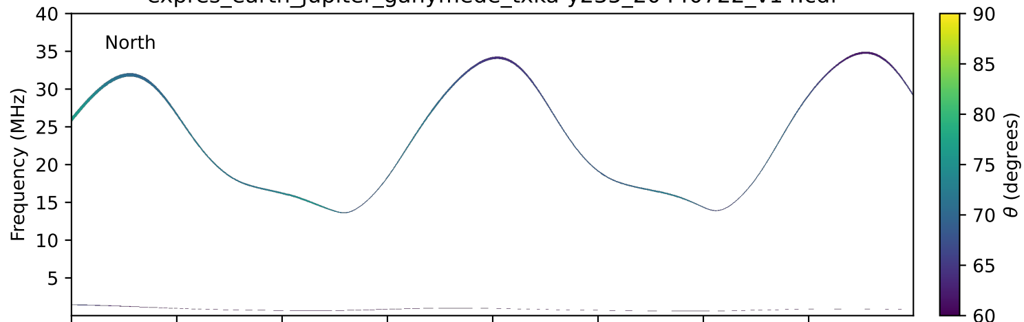
expres_earth_jupiter_ganymede_txka-y235_20440722_v14.cdf
