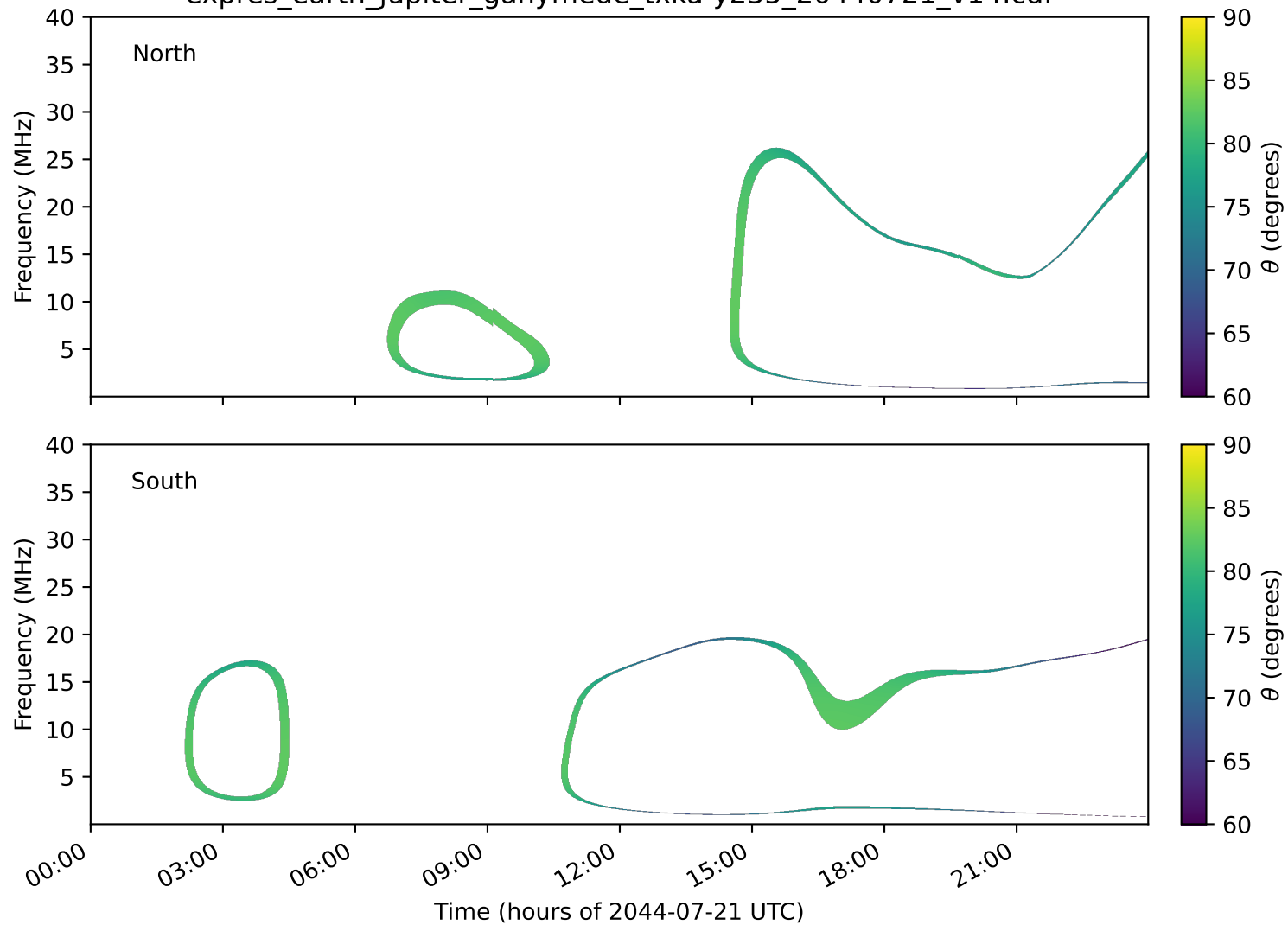
expres_earth_jupiter_ganymede_txka-y235_20440721_v14.cdf
