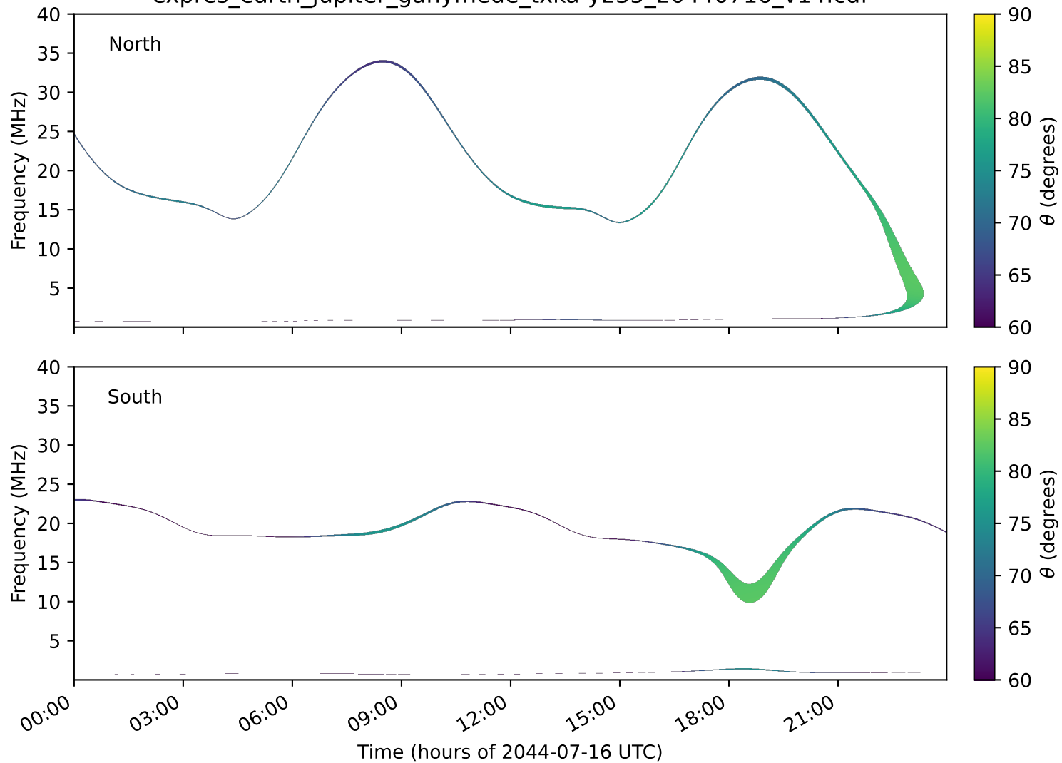
expres_earth_jupiter_ganymede_txka-y235_20440716_v14.cdf
