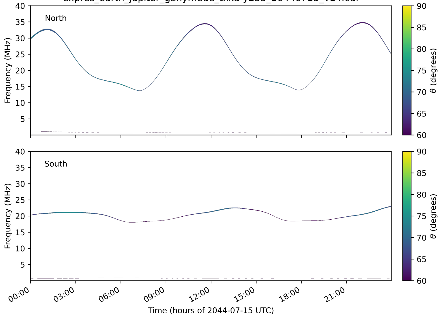
expres_earth_jupiter_ganymede_txka-y235_20440715_v14.cdf
