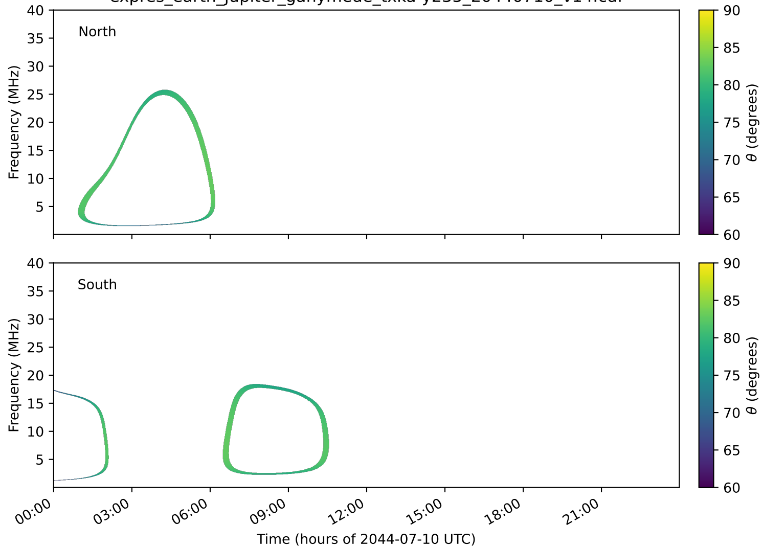
expres_earth_jupiter_ganymede_txka-y235_20440710_v14.cdf
