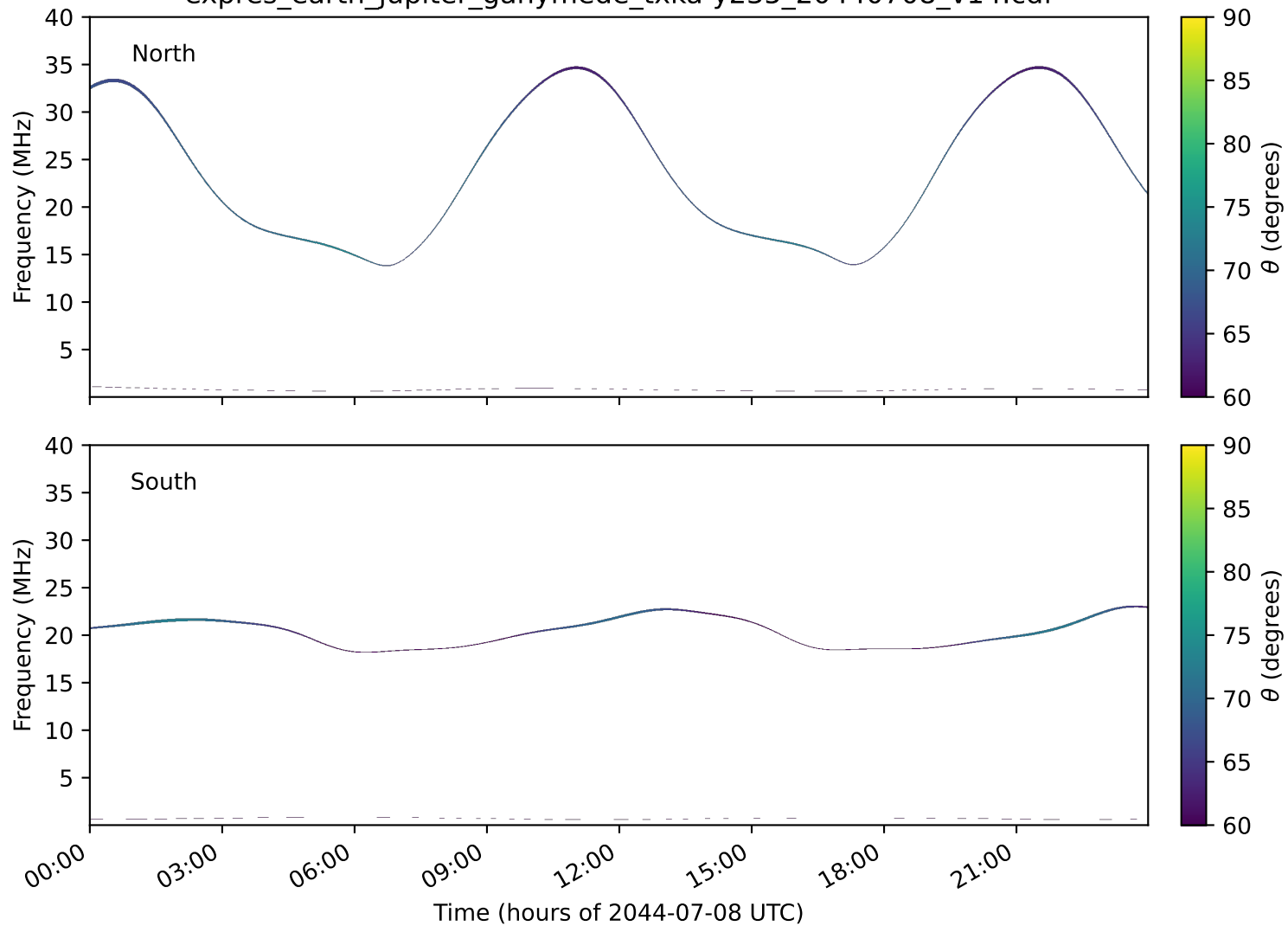
expres_earth_jupiter_ganymede_txka-y235_20440708_v14.cdf
