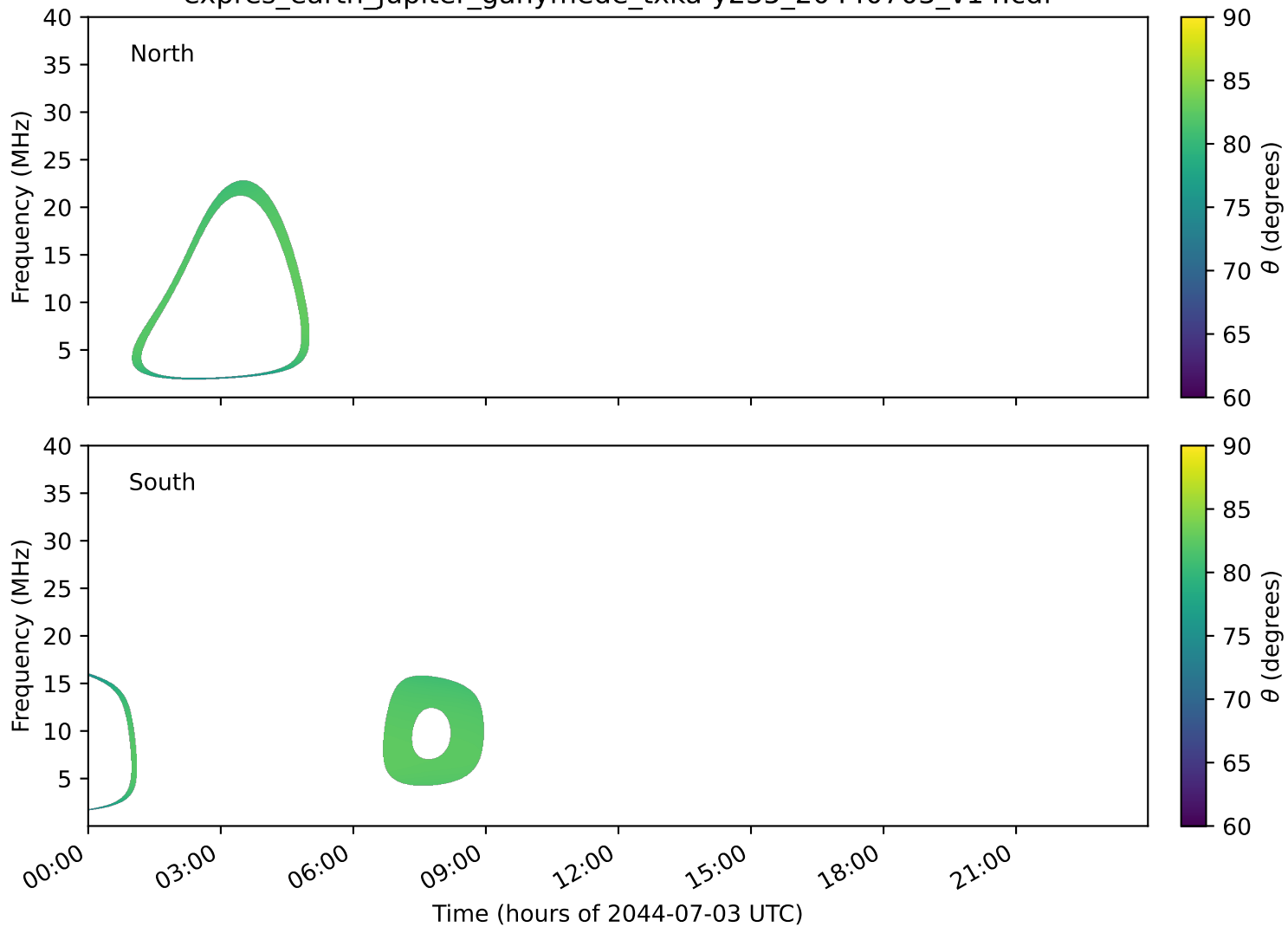
expres_earth_jupiter_ganymede_txka-y235_20440703_v14.cdf
