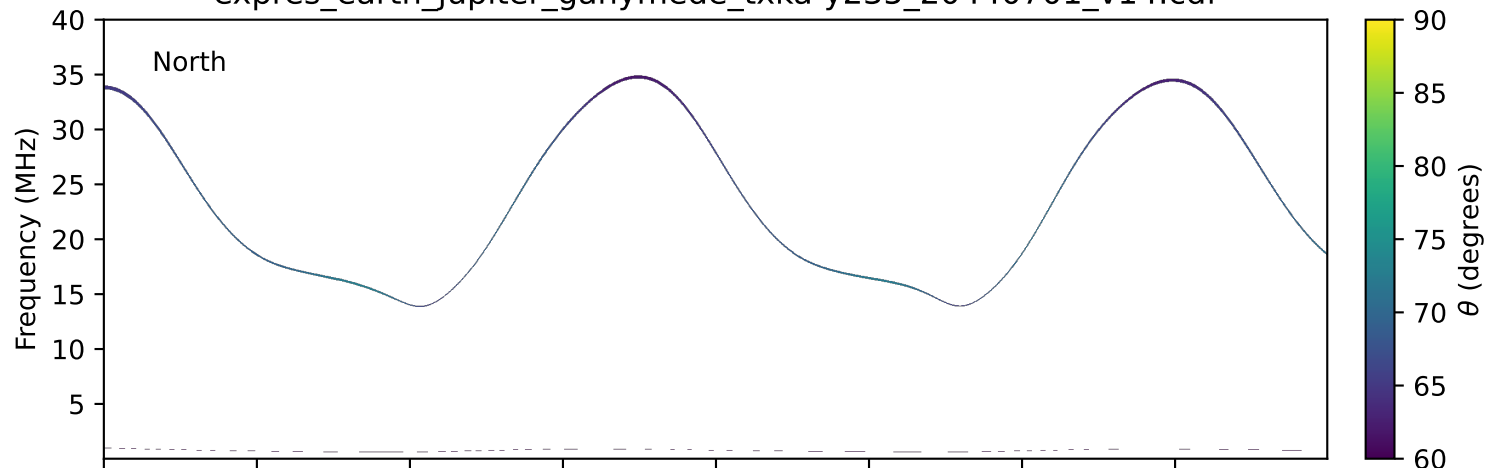
expres_earth_jupiter_ganymede_txka-y235_20440701_v14.cdf
