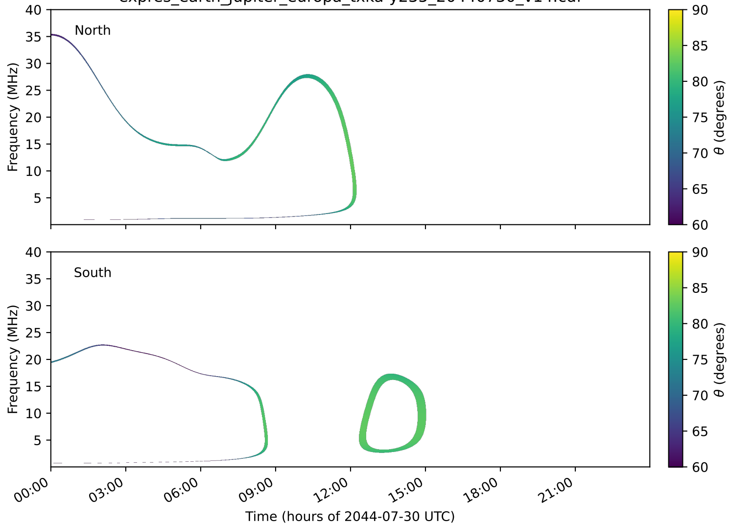
expres_earth_jupiter_europa_txka-y235_20440730_v14.cdf
