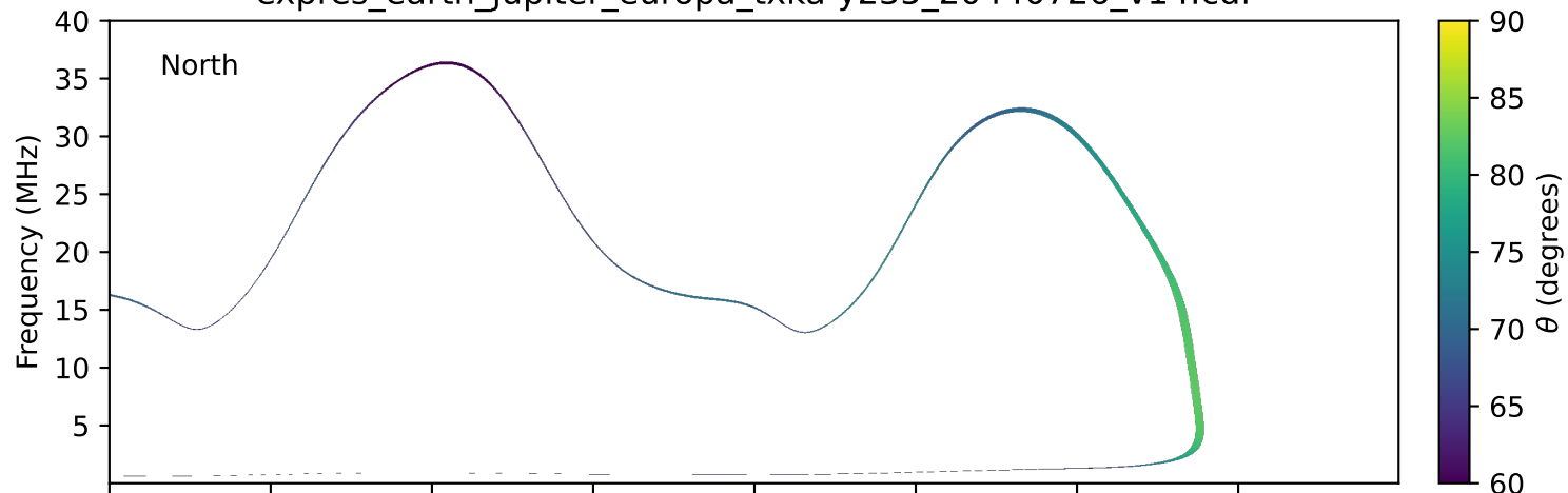
expres_earth_jupiter_europa_txka-y235_20440726_v14.cdf
