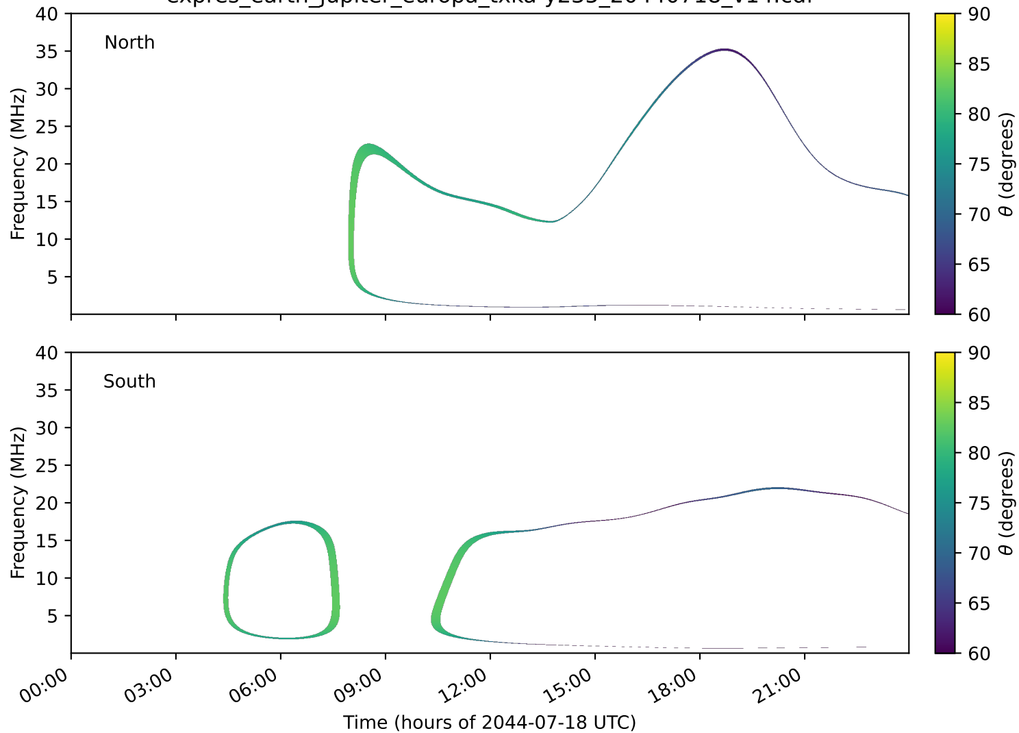
expres_earth_jupiter_europa_txka-y235_20440718_v14.cdf
