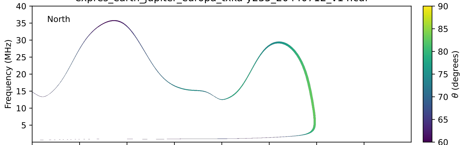
expres_earth_jupiter_europa_txka-y235_20440712_v14.cdf
