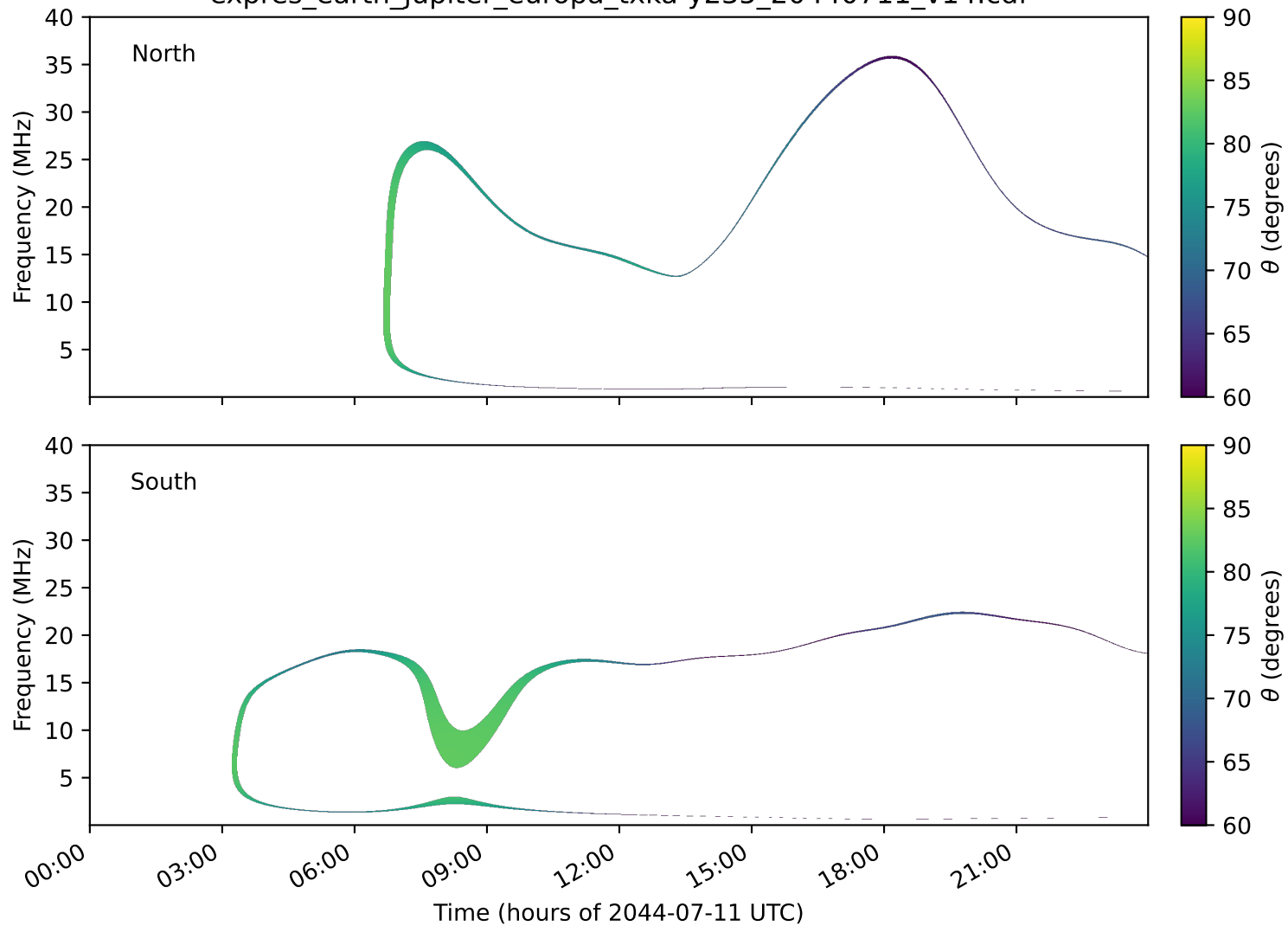
expres_earth_jupiter_europa_txka-y235_20440711_v14.cdf
