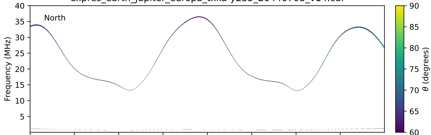
expres_earth_jupiter_europa_txka-y235_20440708_v14.cdf
