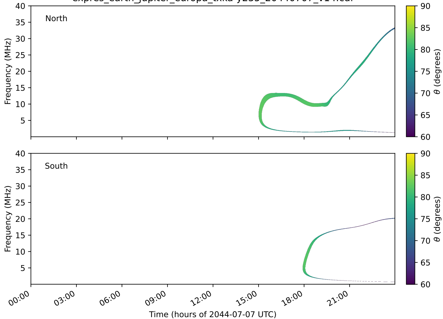
expres_earth_jupiter_europa_txka-y235_20440707_v14.cdf
