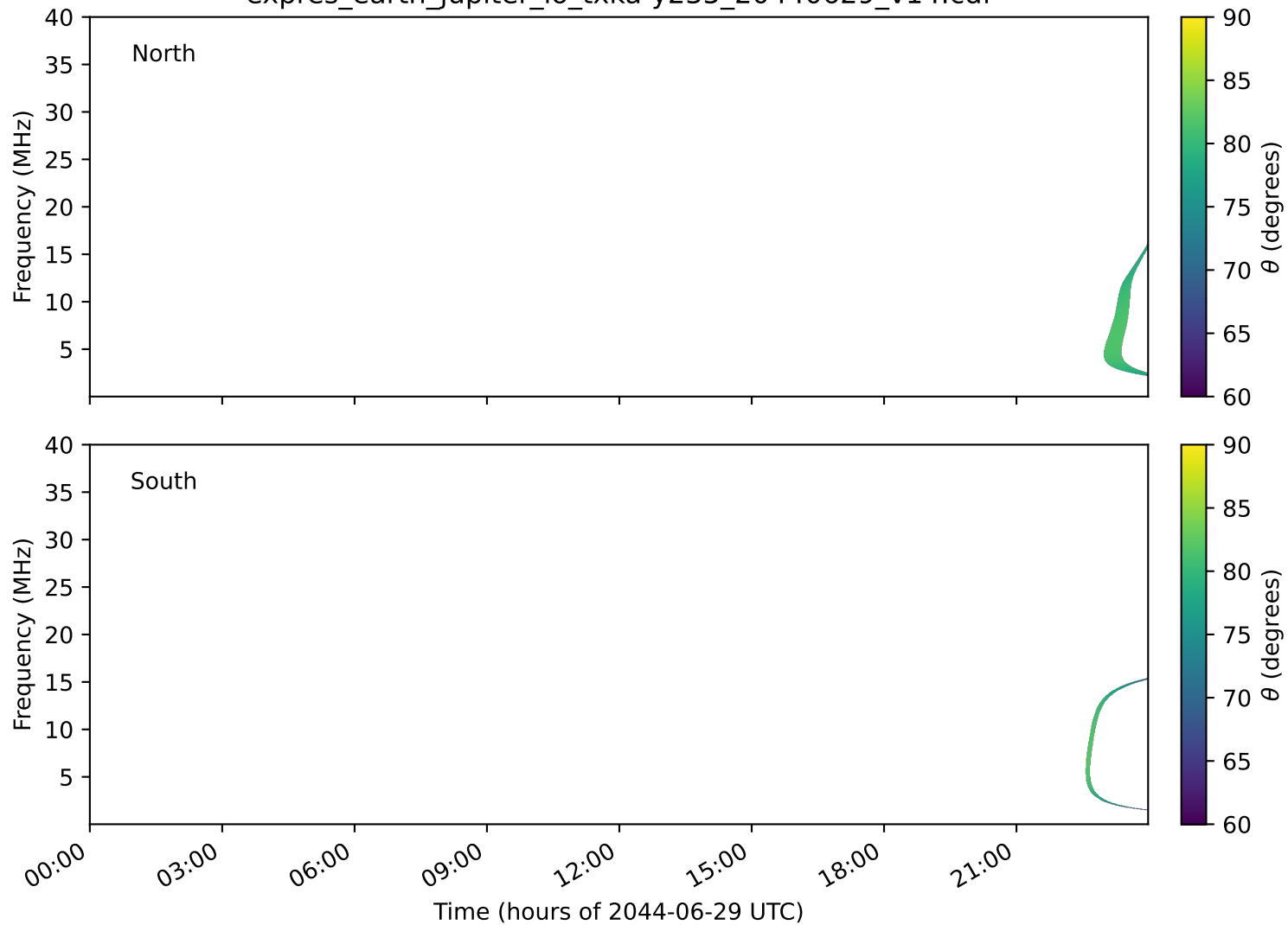
expres_earth_jupiter_io_txka-y235_20440629_v14.cdf
