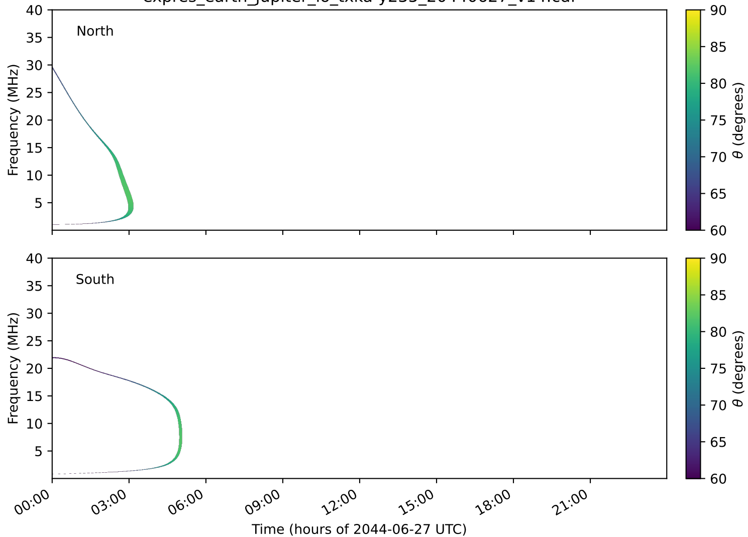
expres_earth_jupiter_io_txka-y235_20440627_v14.cdf
