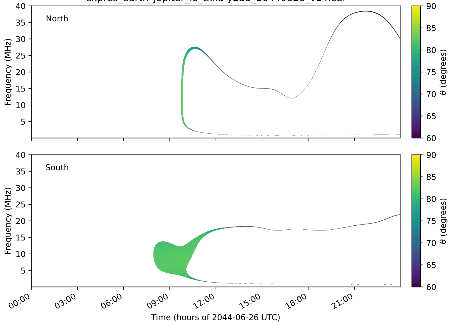
expres_earth_jupiter_io_txka-y235_20440626_v14.cdf
