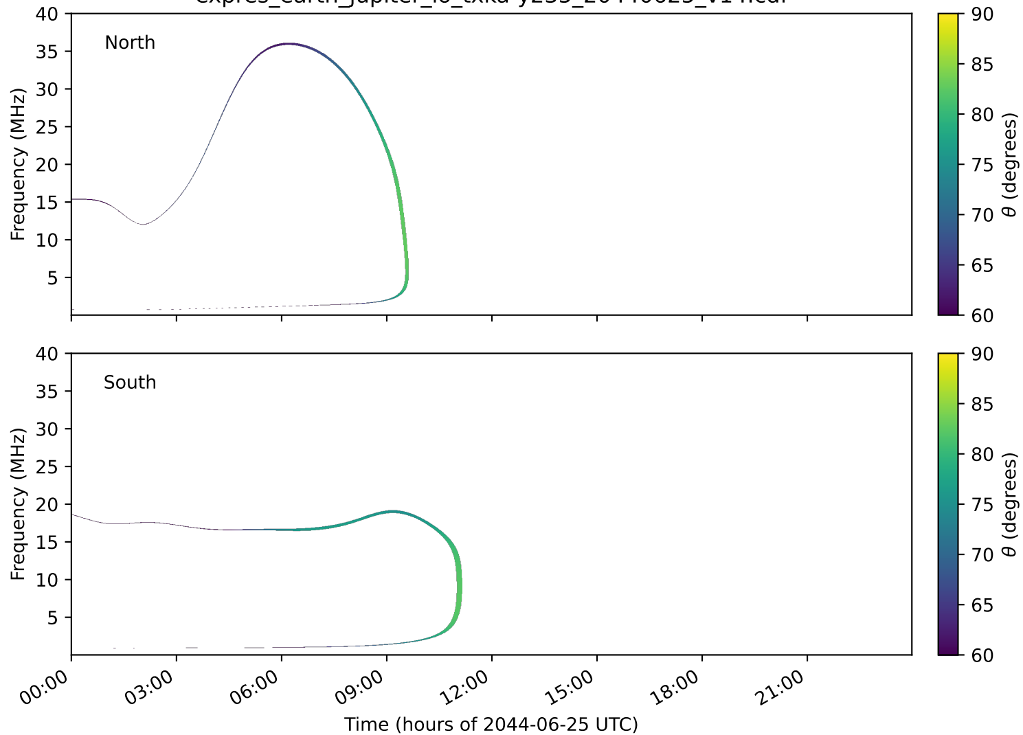
expres_earth_jupiter_io_txka-y235_20440625_v14.cdf
