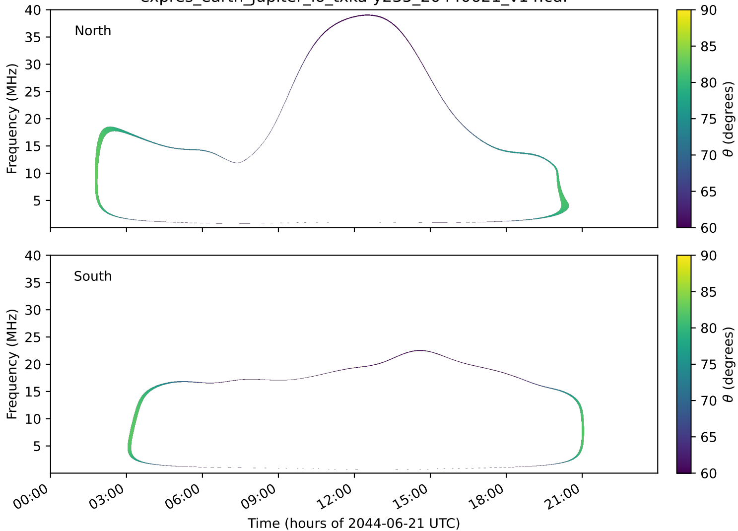
expres_earth_jupiter_io_txka-y235_20440621_v14.cdf
