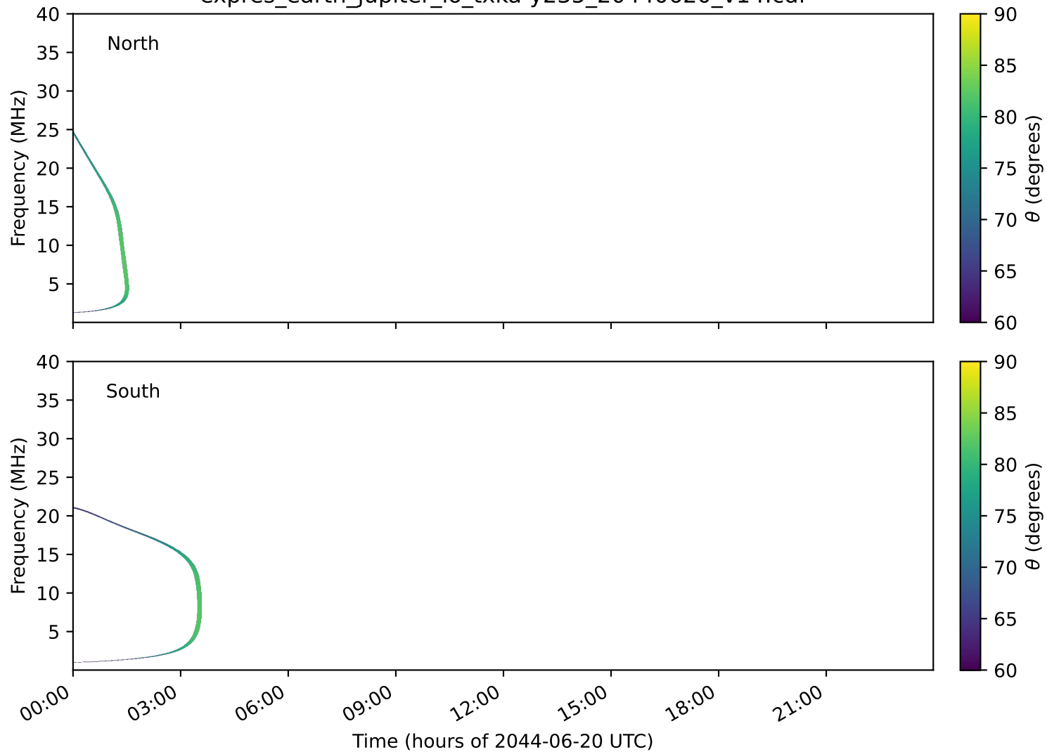
expres_earth_jupiter_io_txka-y235_20440620_v14.cdf
