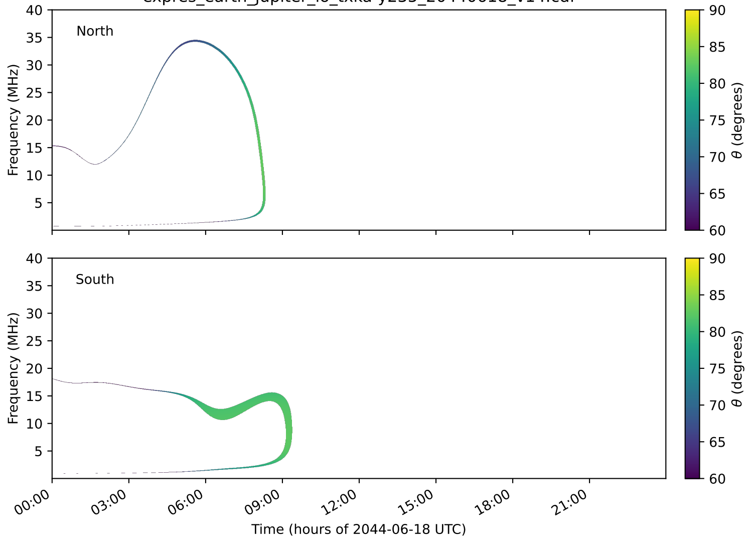
expres_earth_jupiter_io_txka-y235_20440618_v14.cdf
