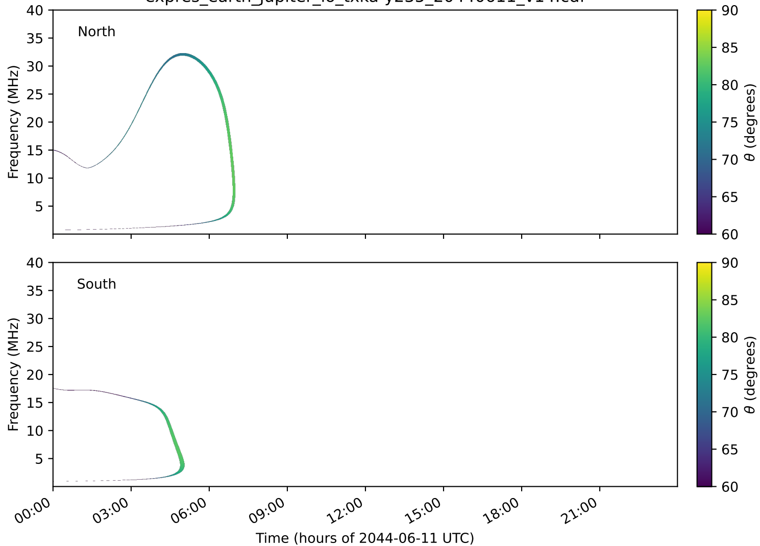
expres_earth_jupiter_io_txka-y235_20440611_v14.cdf
