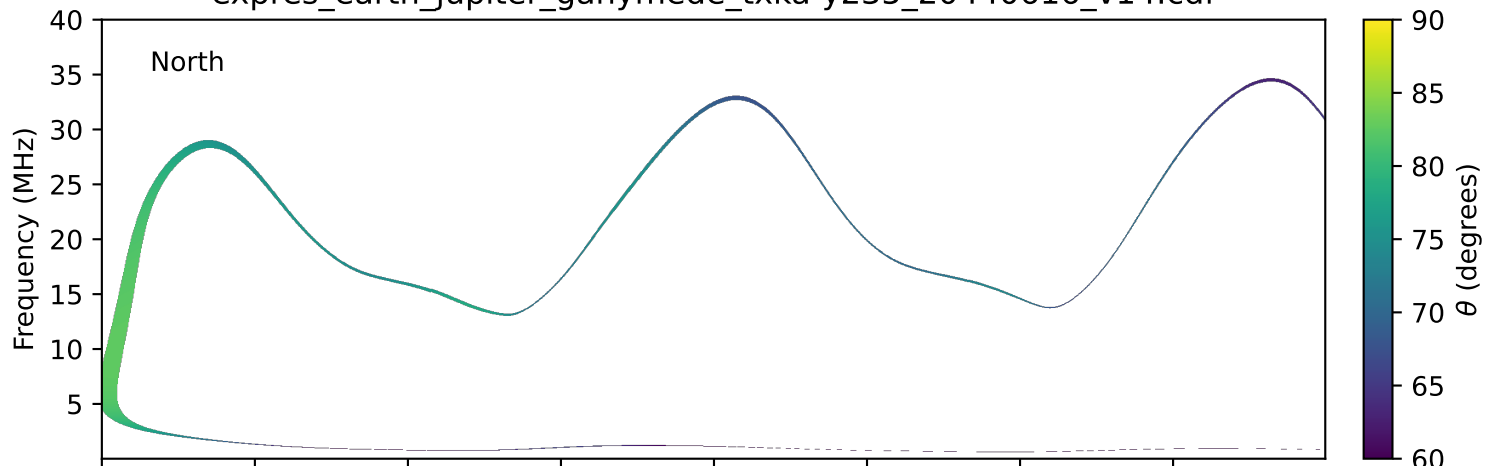
expres_earth_jupiter_ganymede_txka-y235_20440616_v14.cdf
