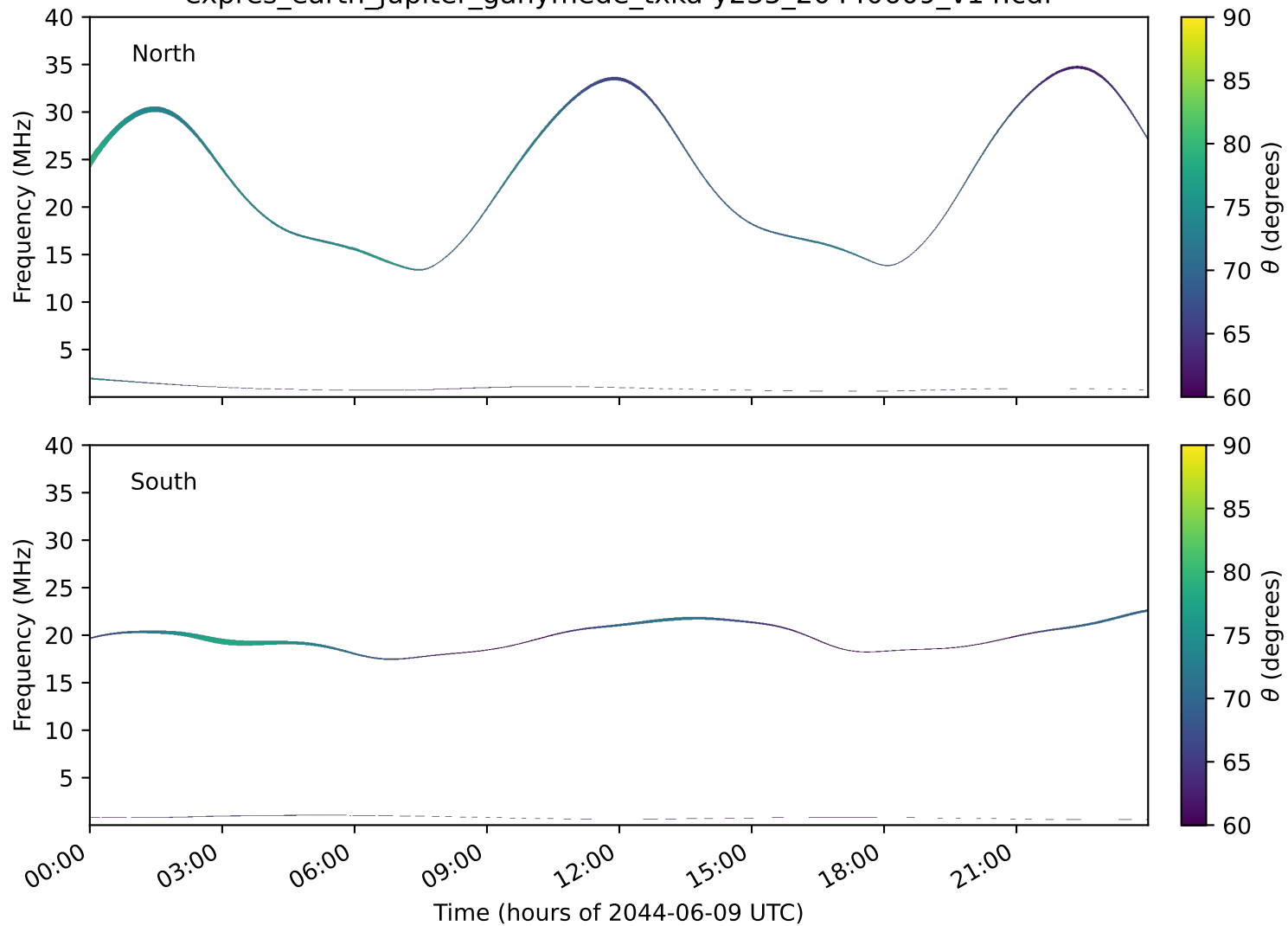
expres_earth_jupiter_ganymede_txka-y235_20440609_v14.cdf
