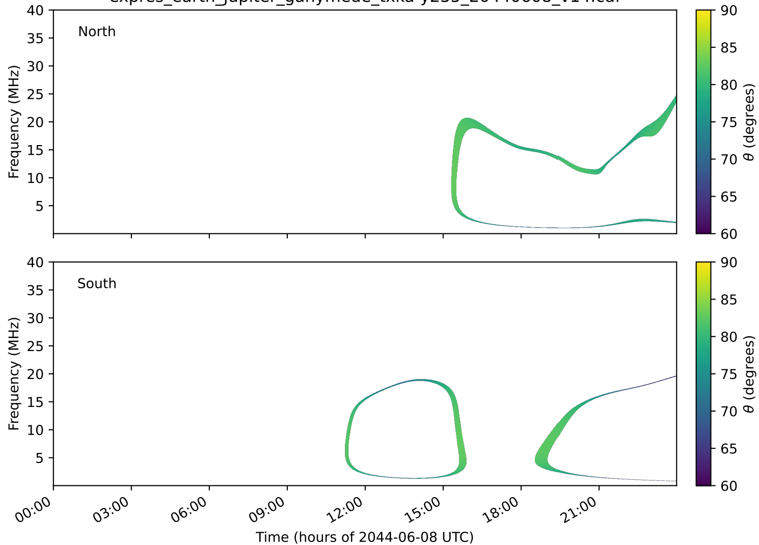
expres_earth_jupiter_ganymede_txka-y235_20440608_v14.cdf
