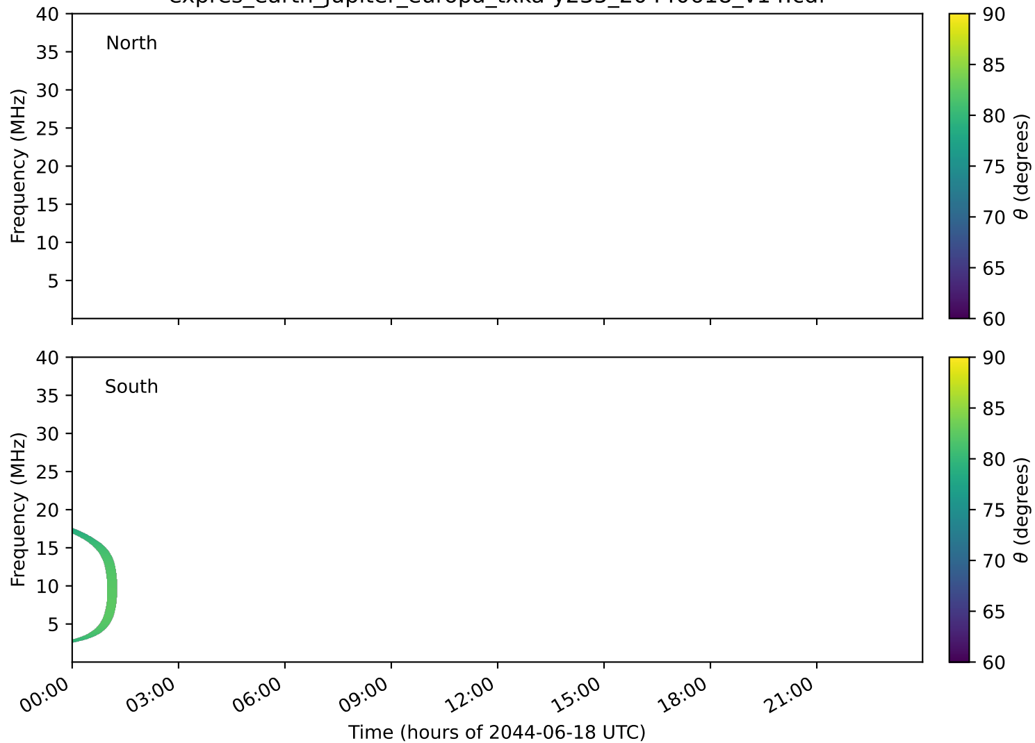
expres_earth_jupiter_europa_txka-y235_20440618_v14.cdf
