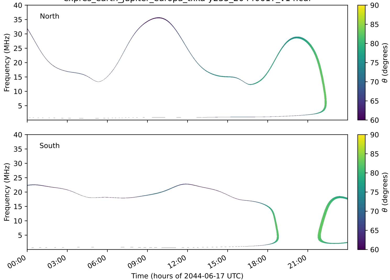
expres_earth_jupiter_europa_txka-y235_20440617_v14.cdf
