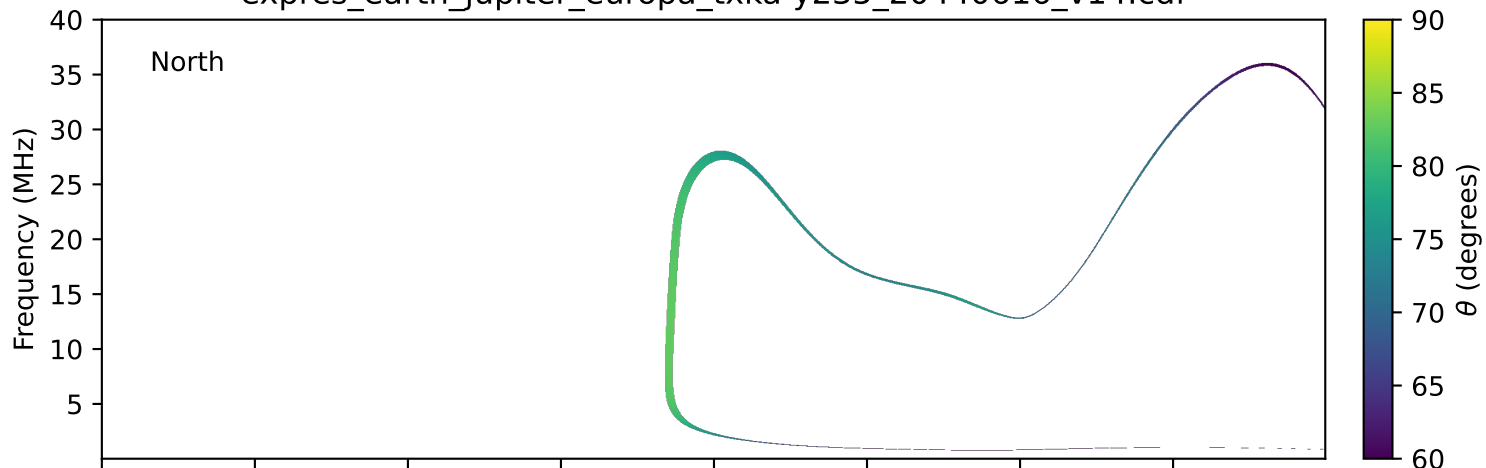
expres_earth_jupiter_europa_txka-y235_20440616_v14.cdf
