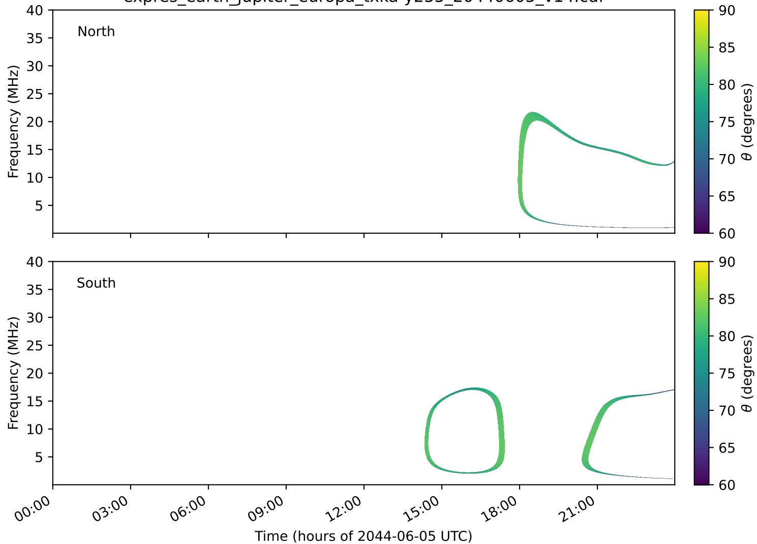
expres_earth_jupiter_europa_txka-y235_20440605_v14.cdf
