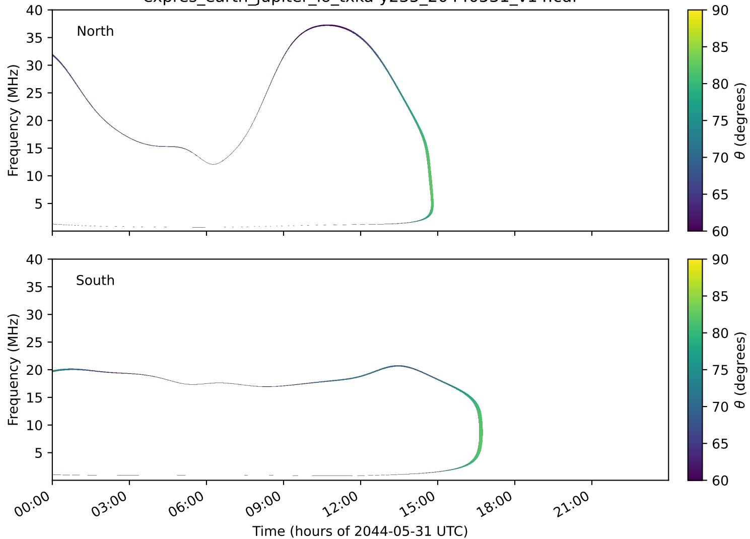
expres_earth_jupiter_io_txka-y235_20440531_v14.cdf
