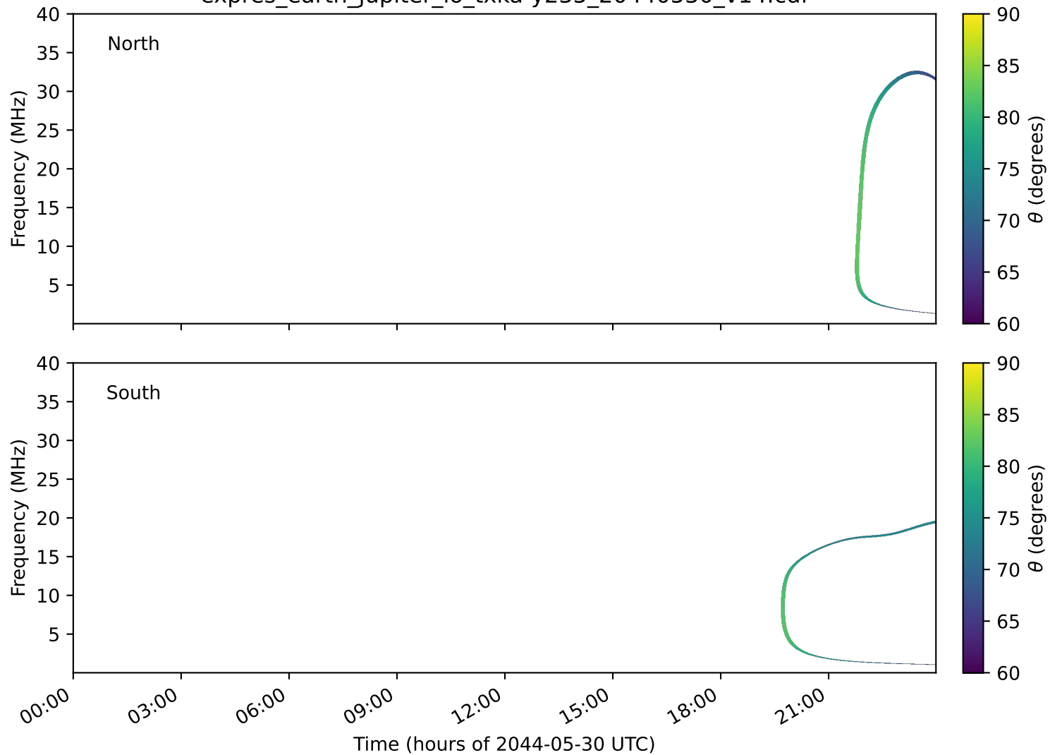
expres_earth_jupiter_io_txka-y235_20440530_v14.cdf
