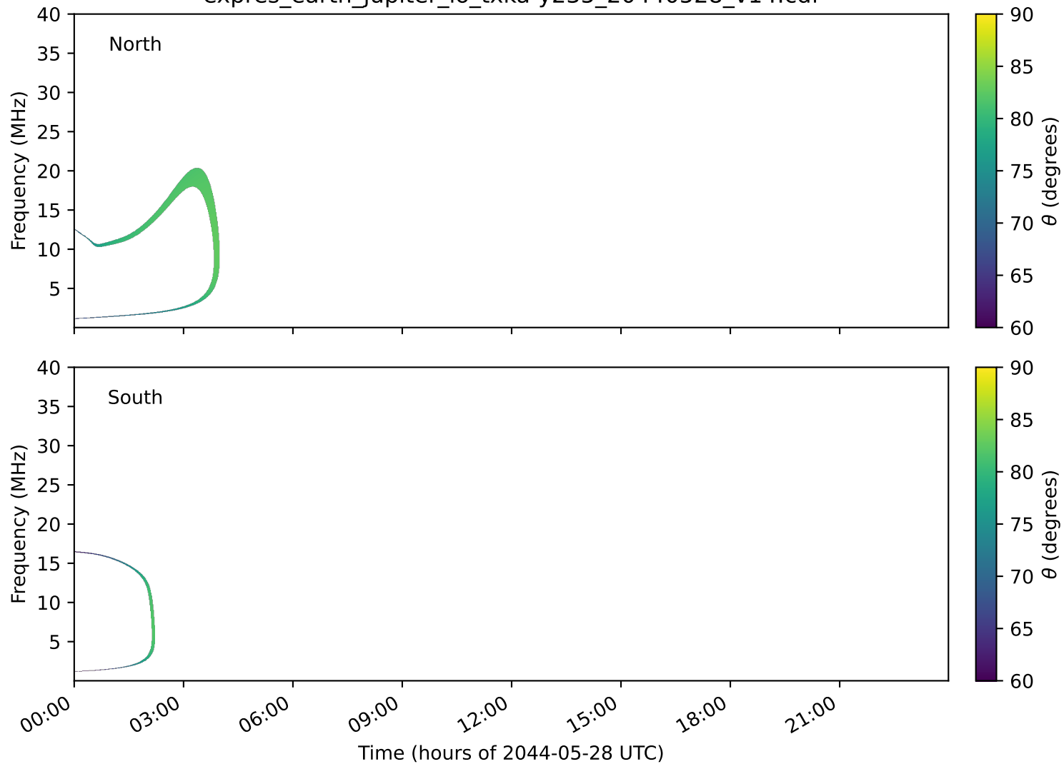
expres_earth_jupiter_io_txka-y235_20440528_v14.cdf
