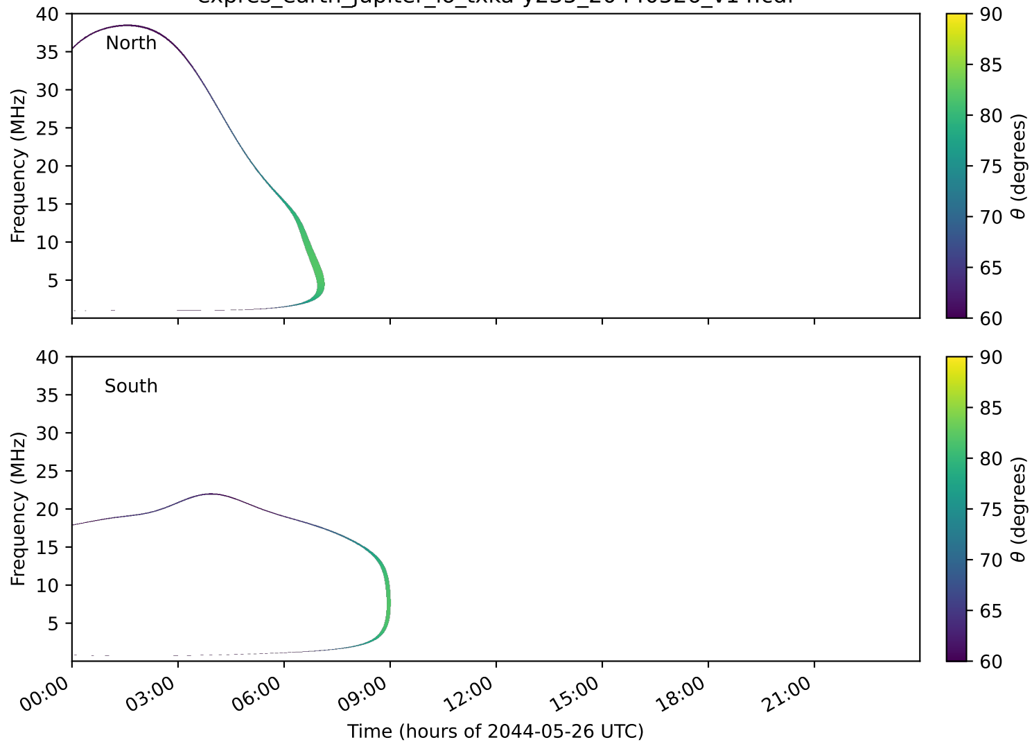
expres_earth_jupiter_io_txka-y235_20440526_v14.cdf
