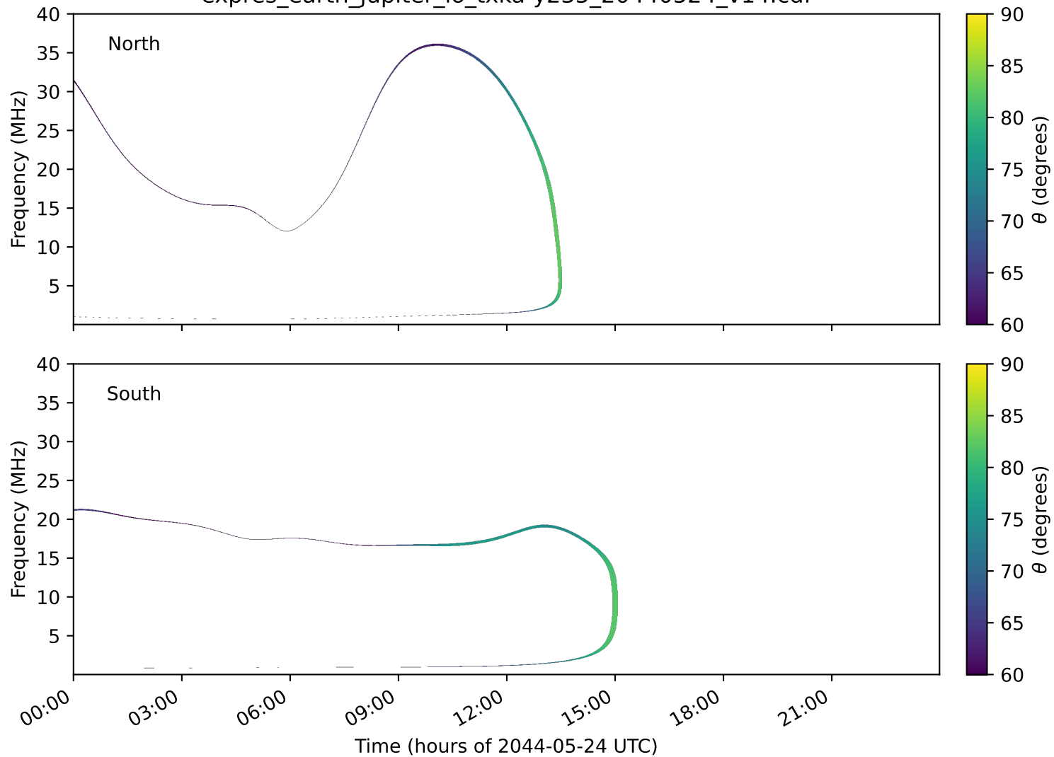
expres_earth_jupiter_io_txka-y235_20440524_v14.cdf
