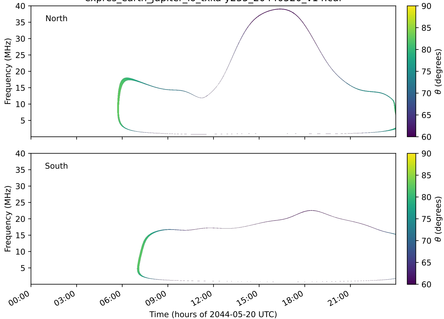
expres_earth_jupiter_io_txka-y235_20440520_v14.cdf
