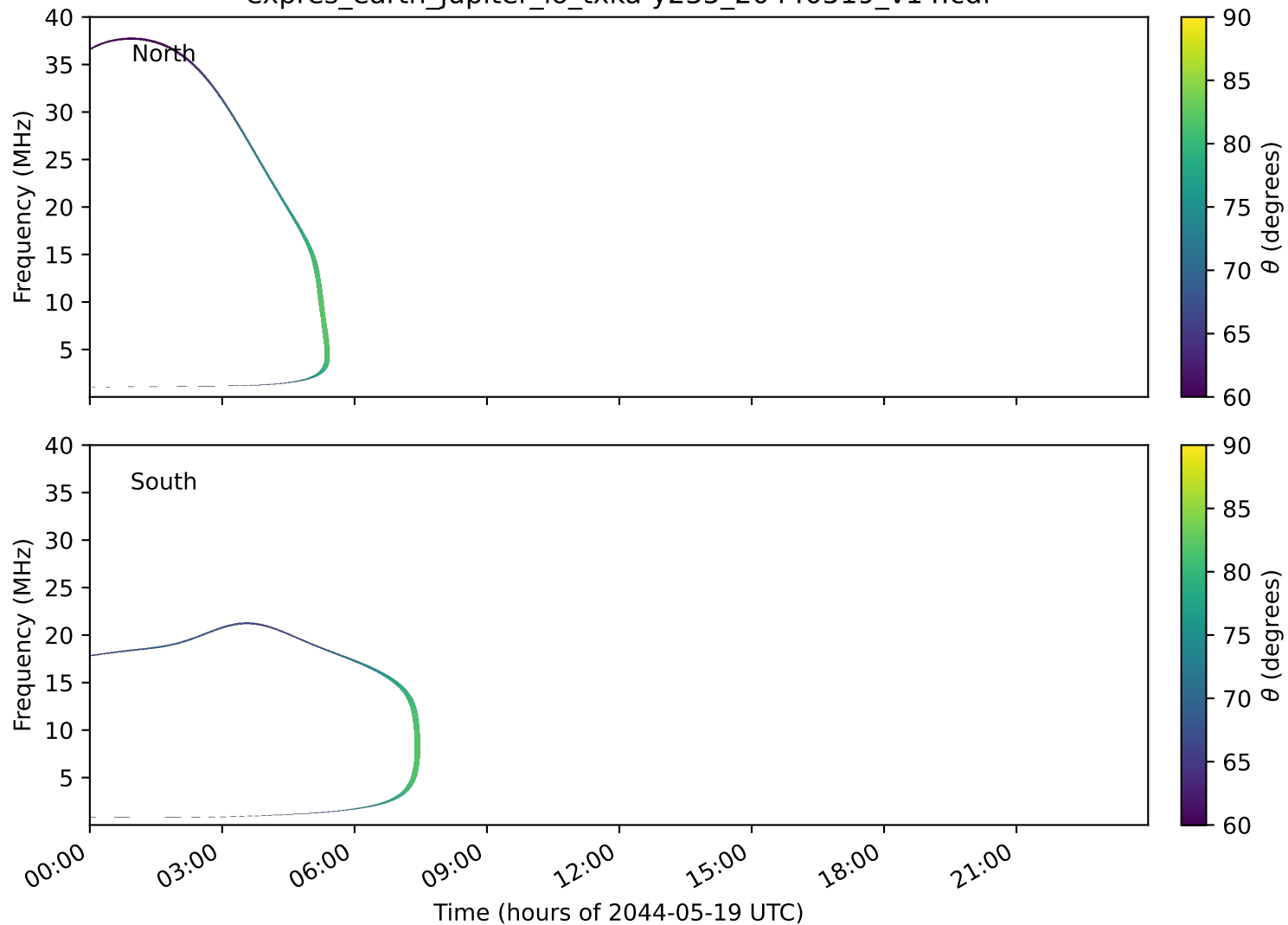
expres_earth_jupiter_io_txka-y235_20440519_v14.cdf
