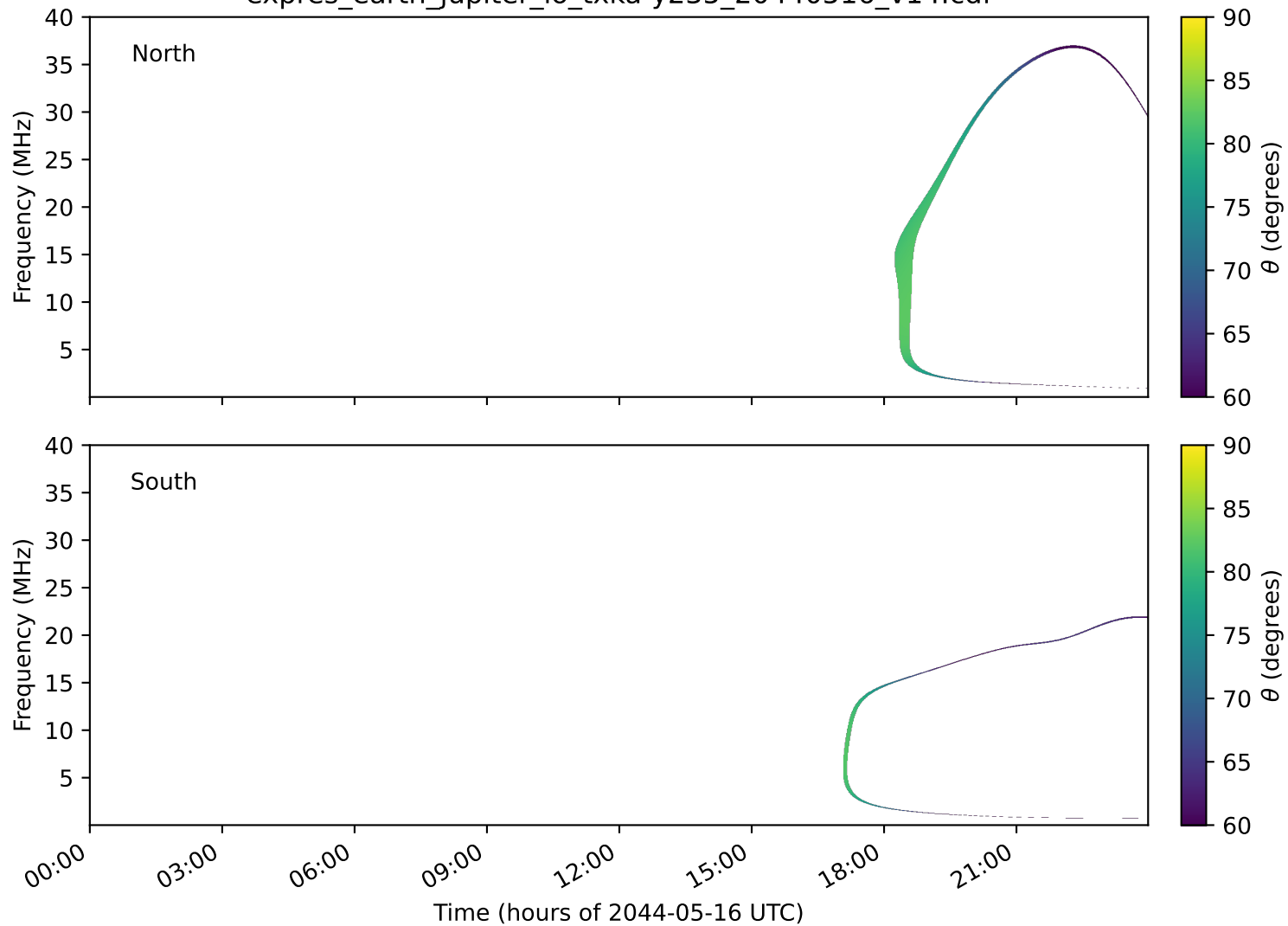
expres_earth_jupiter_io_txka-y235_20440516_v14.cdf
