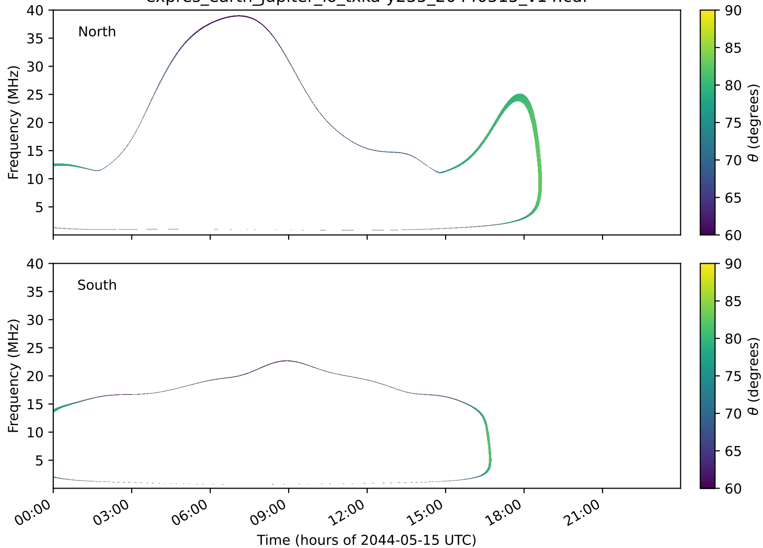
expres_earth_jupiter_io_txka-y235_20440515_v14.cdf
