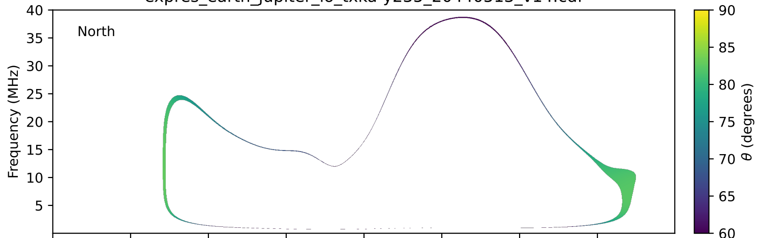
expres_earth_jupiter_io_txka-y235_20440513_v14.cdf
