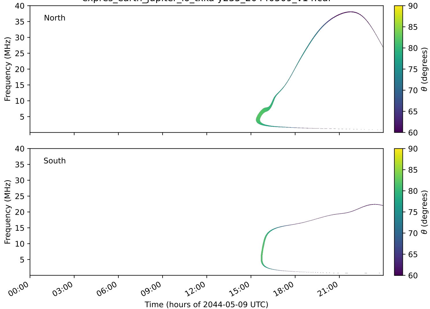
expres_earth_jupiter_io_txka-y235_20440509_v14.cdf
