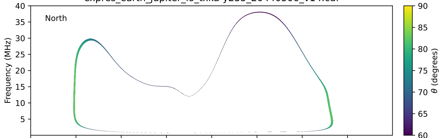
expres_earth_jupiter_io_txka-y235_20440506_v14.cdf
