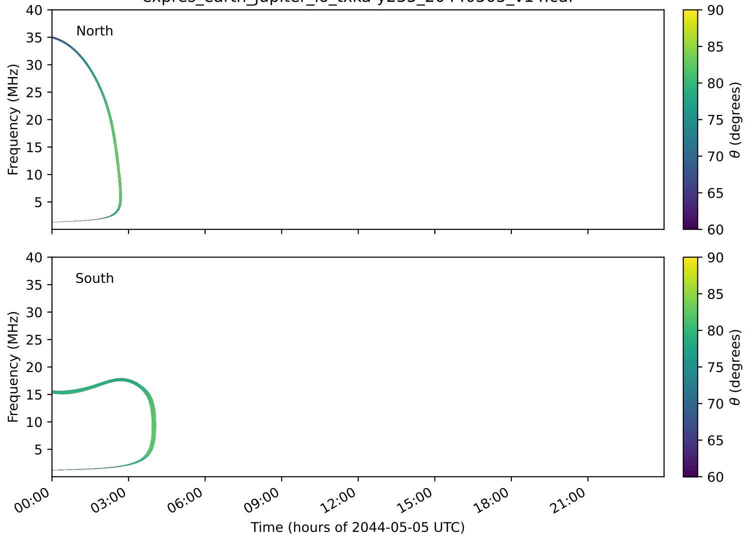
expres_earth_jupiter_io_txka-y235_20440505_v14.cdf
