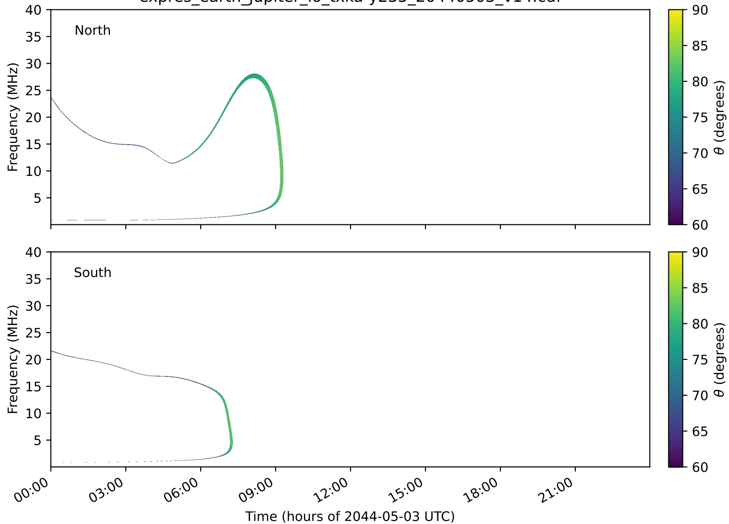
expres_earth_jupiter_io_txka-y235_20440503_v14.cdf
