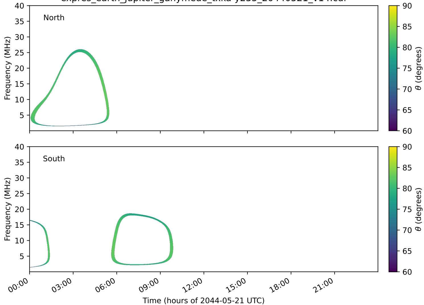
expres_earth_jupiter_ganymede_txka-y235_20440521_v14.cdf
