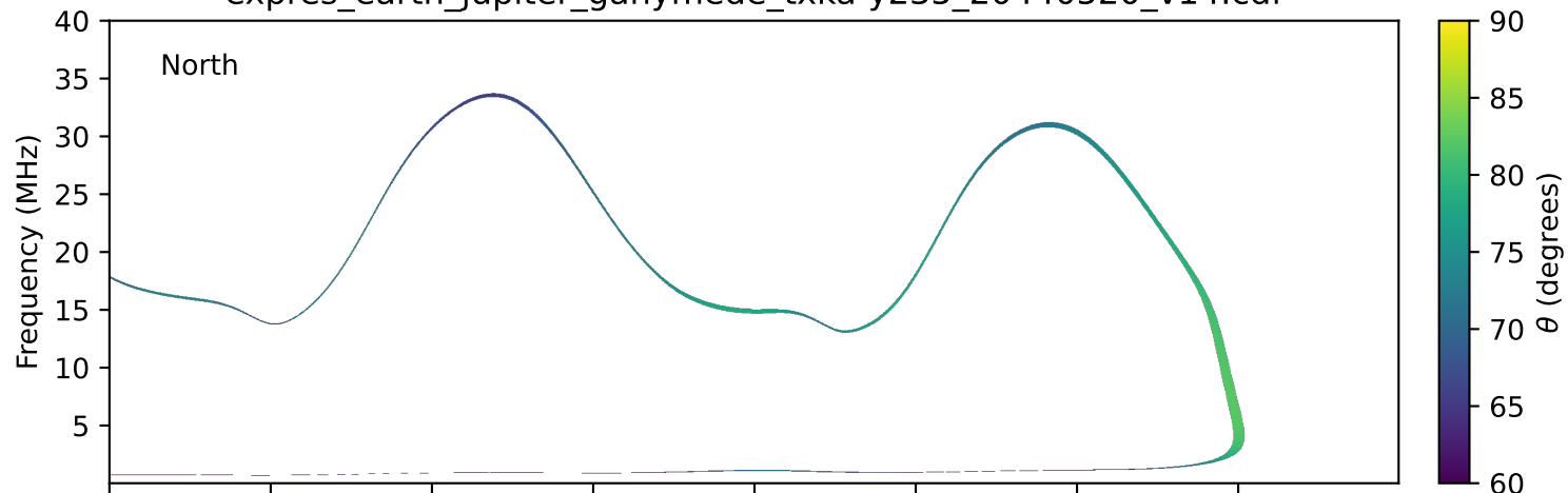
expres_earth_jupiter_ganymede_txka-y235_20440520_v14.cdf
