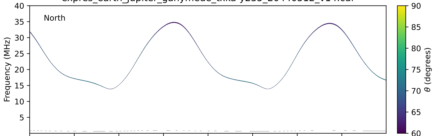
expres_earth_jupiter_ganymede_txka-y235_20440512_v14.cdf
